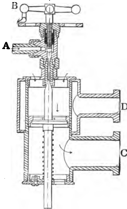
FIG. 318.—The Huzelstein Carburetter. A is the inlet for gasoline; B, the valve controlling inlet; C, the tube leading to cylinder combustion space; D, tube for leading hot exhaust gases around the jacket on the mixing chamber. Arrows indicate entrance for air and course of mixture to cylinder.
